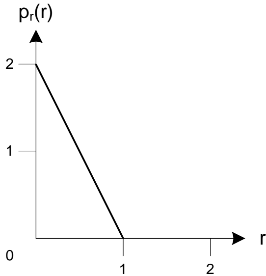
Original probability density function
