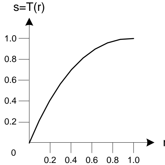
Transformation function
