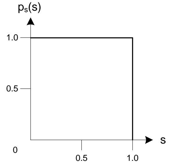
Resulting uniform density
